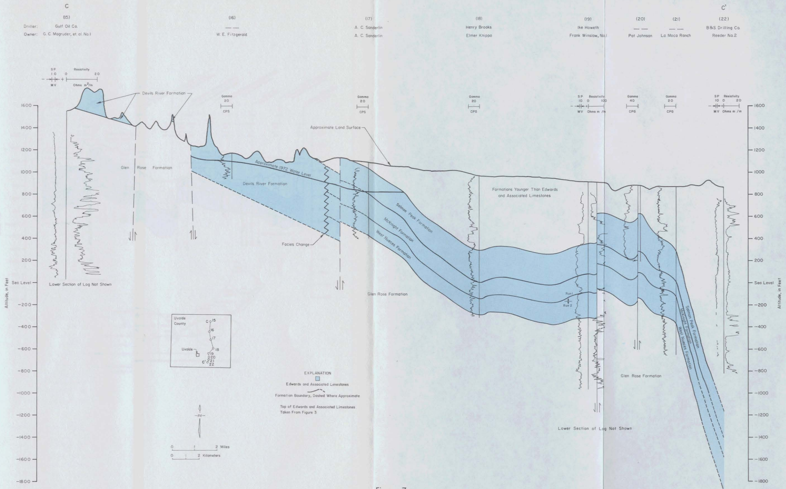
Figure 7 Geohydrologic Section C-C'
