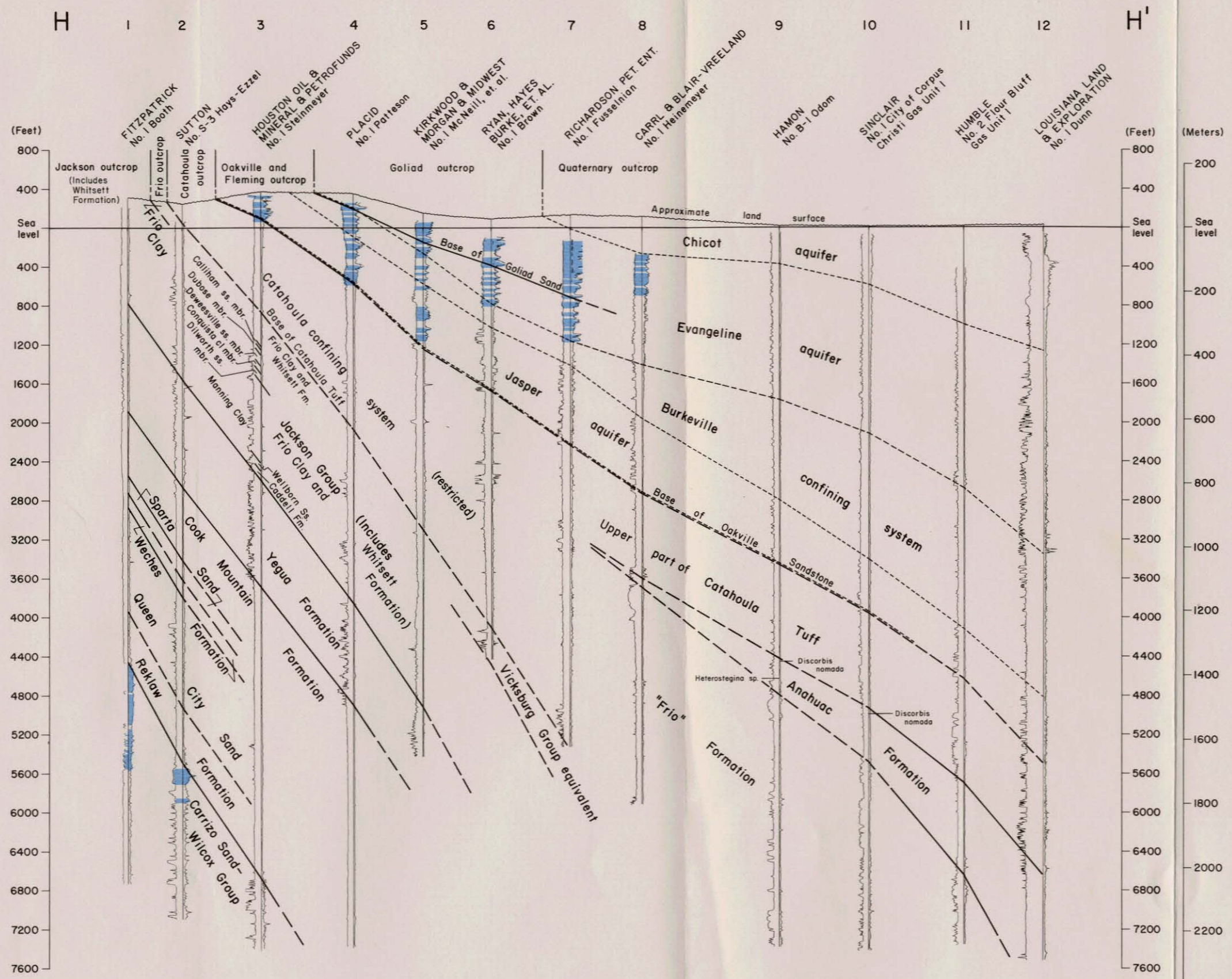
Figure 9 Stratigraphic and Hydrogeologic Section H-H'
