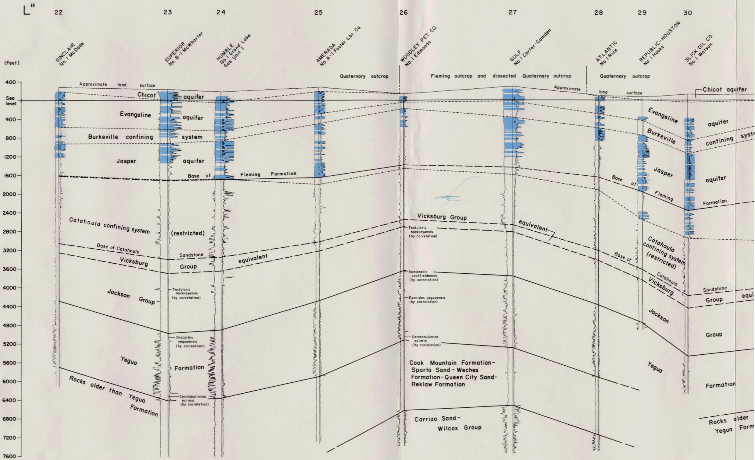
Figure 15 Stratigraphic and Hydrogeologic Section L''-L'''
