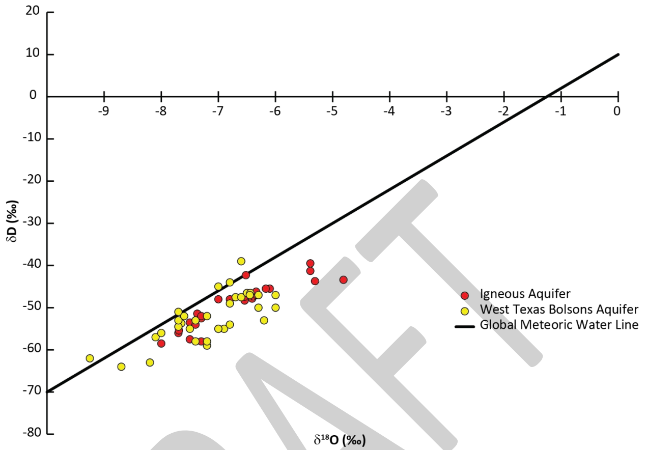
Figure 4.7.12. Groundwater stable oxygen isotopes ( \delta^{18}\text{O} , in per mil) and stable hydrogen isotopes ( \delta^2\text{H} , in per mil) in the Igneous and West Texas Bolsons aquifers (data from TWDB, 2022a).
