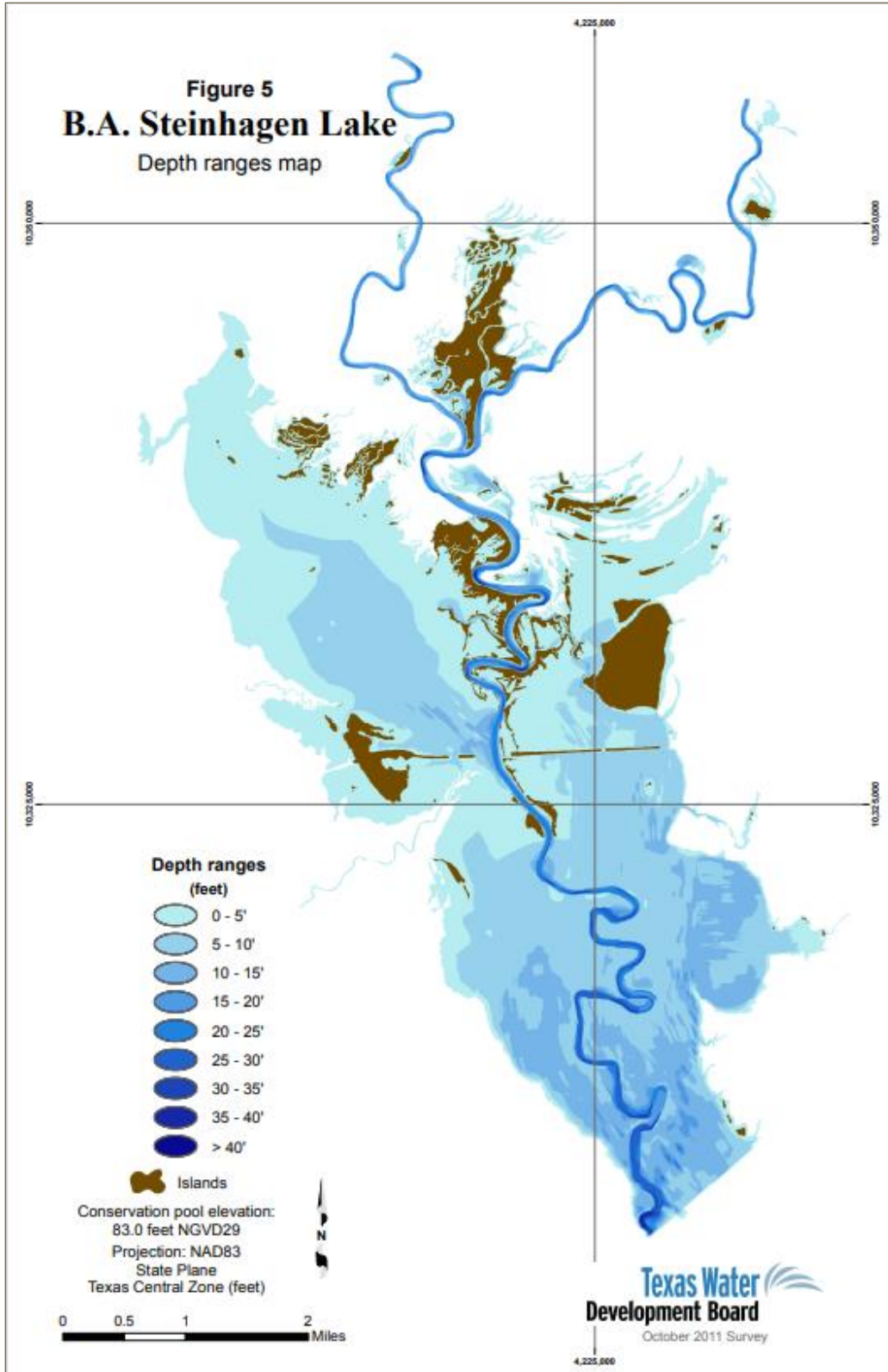
FIGURE 2-12: DEPTH RANGES MAP FOR B.A. STEINHAGEN LAKE (Source: Volumetric and Sedimentation Survey of B.A. Steinhagen Lake, TWDB, 2011)
