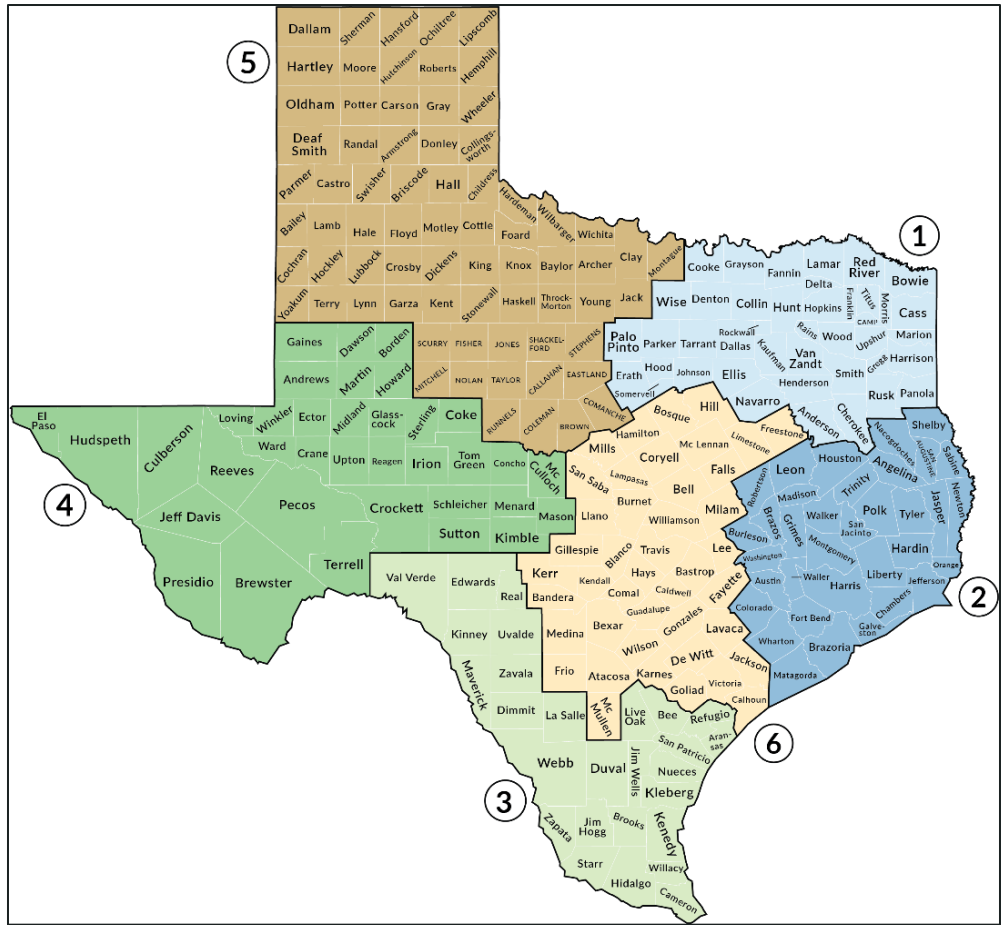
FIGURE 7-2: TDEM REGIONS
